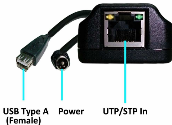
UB-101R Receiver (Remote)
